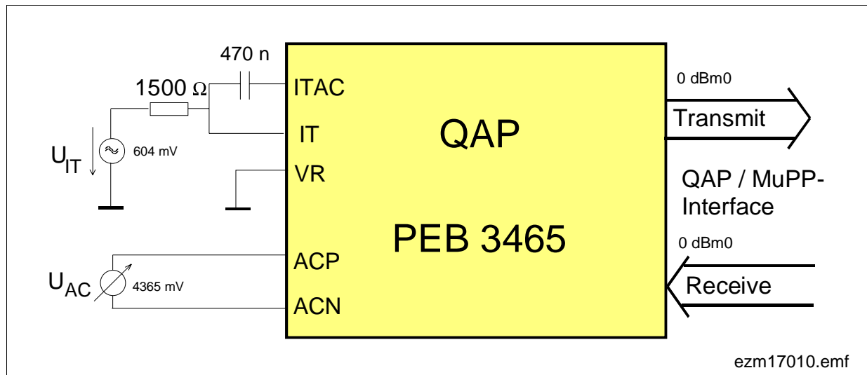
Figure 9 Transmission Characteristics
