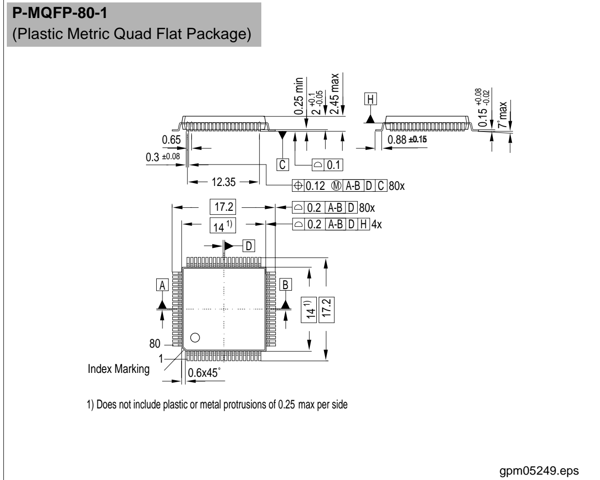
Figure 20 Package Outline: PEB 3465 (QAP)
