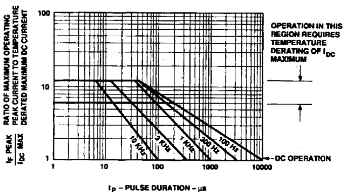
Figure 1. Maximum Tolerable Peak Current vs. Pulse Duration - Red.
