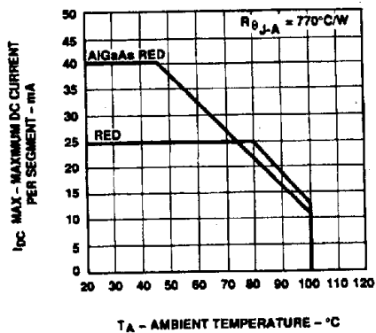
Figure 3. Maximum Allowable DC Current vs. Ambient Temperature.
