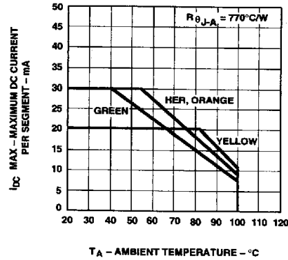
Figure 10. Maximum Allowable DC Current vs. Ambient Temperature.
