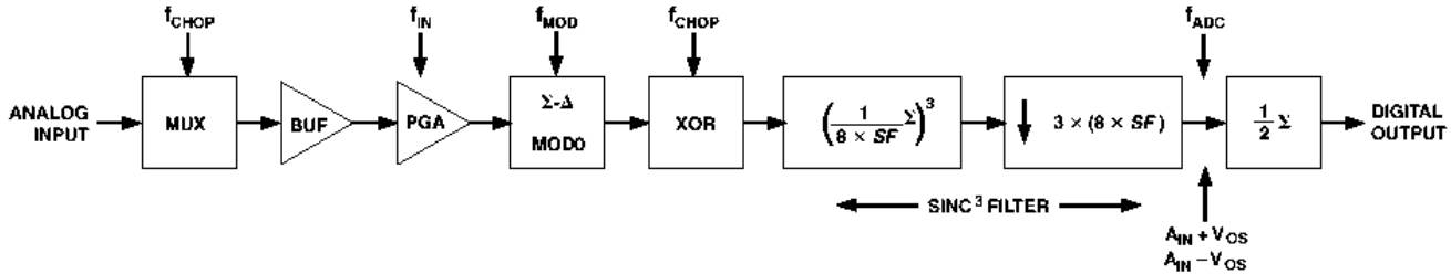
Figure 7: ADC Circuit Diagram with Chopping Enabled
