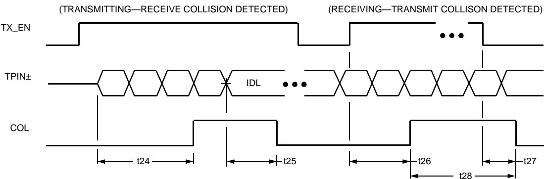
Figure 16. Serial 10 Mb/s Timing for TX_EN, TPIN, and COL
