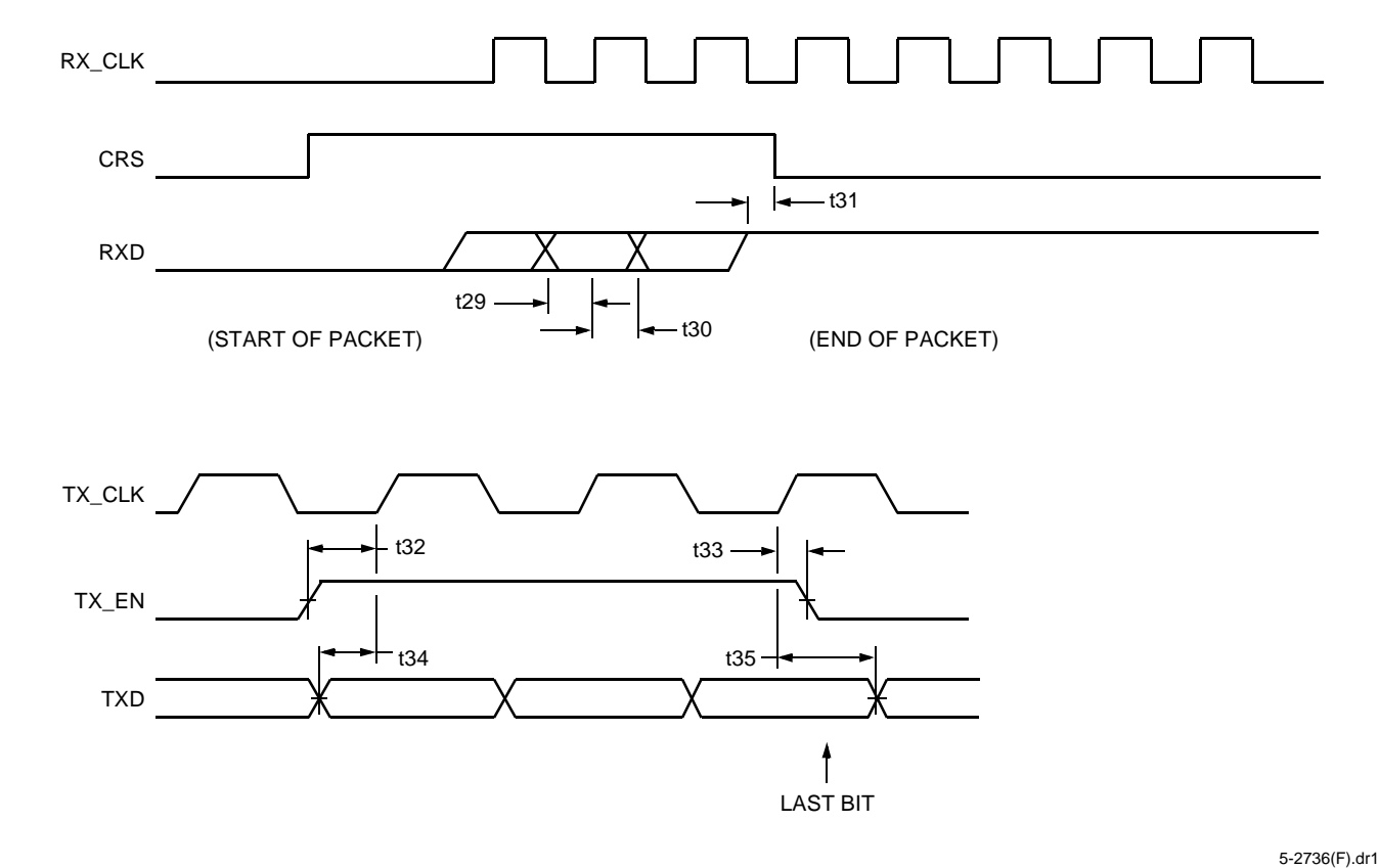
Figure 17. Serial 10 Mbits/s Timing for RX_CLK, CRS, RXD, TX_CLK, TX_EN, and TXD
