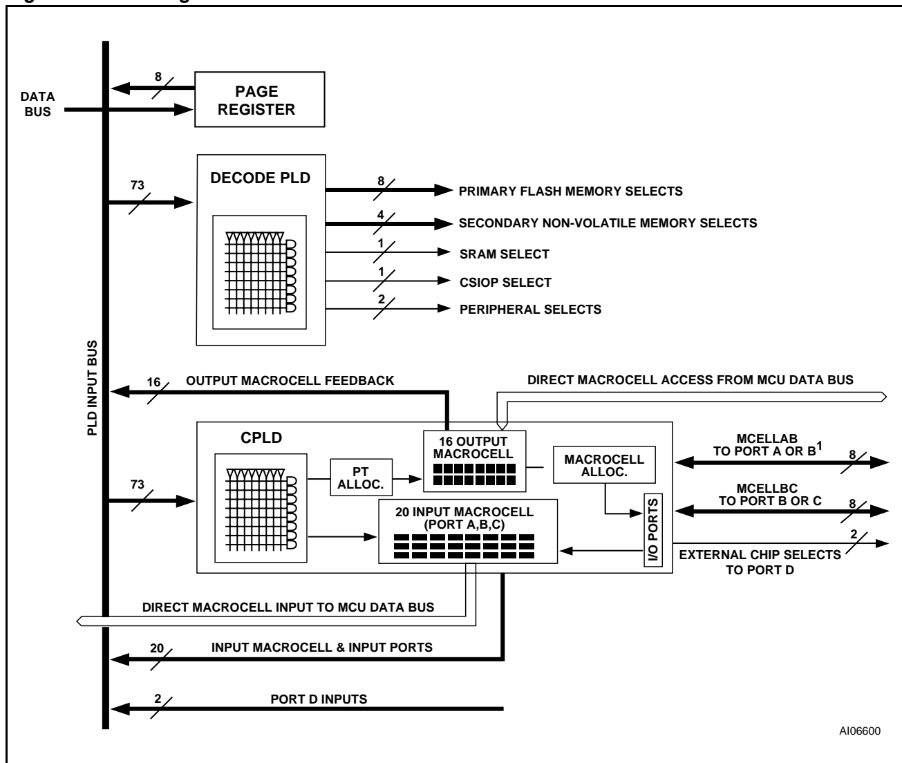
Figure 58. PLD Diagram
