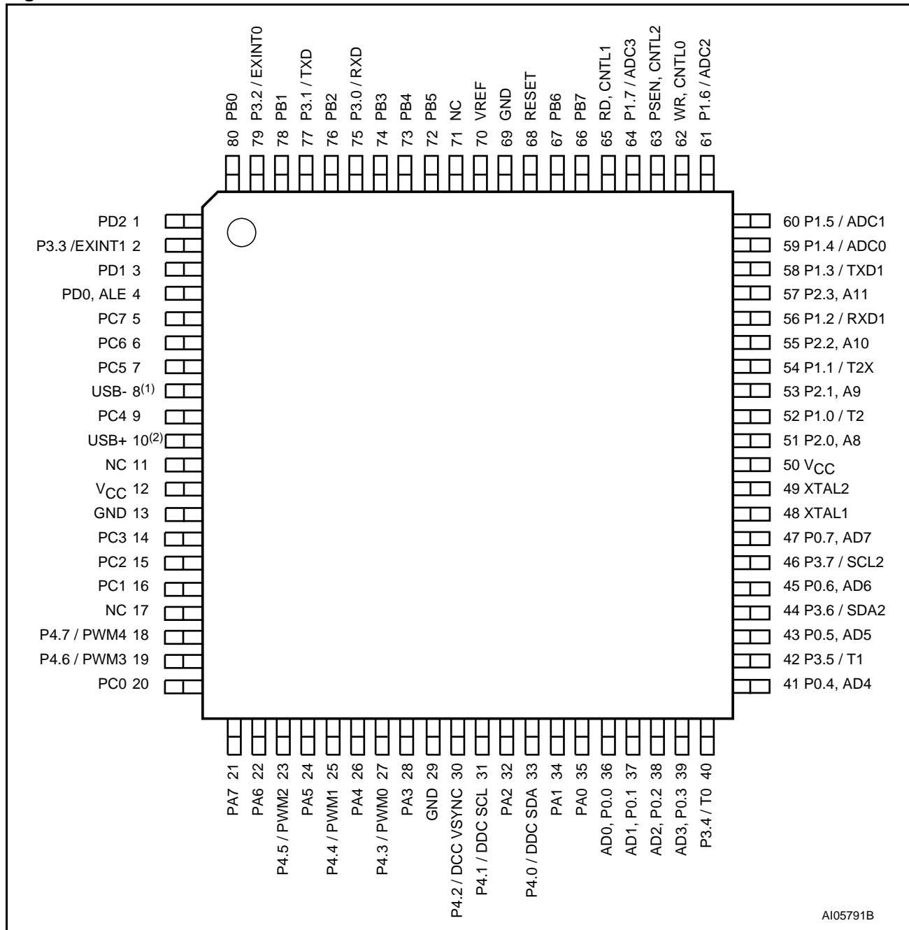
Figure 4. TQFP80 Connections
