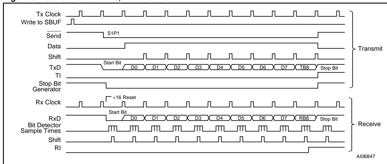
Figure 34. Serial Port Mode 3, Waveforms
