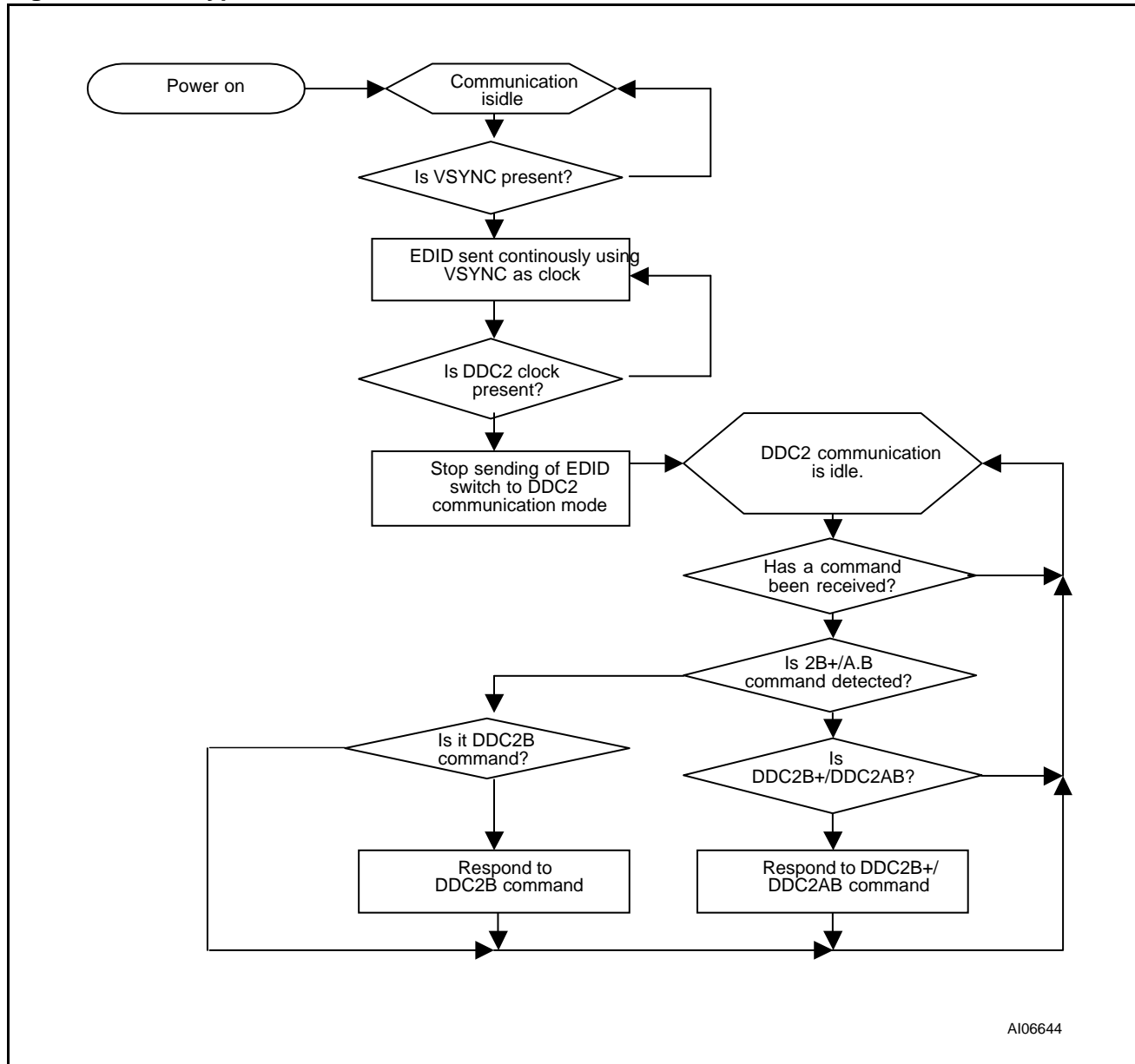
Figure 41. Host Type Detection
