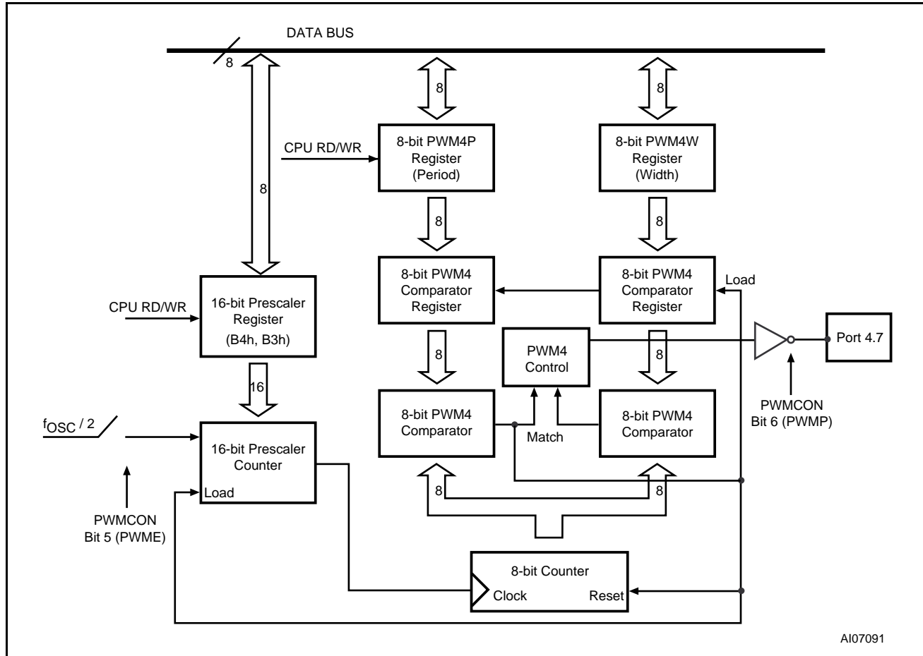
Figure 37. Programmable PWM 4 Channel Block Diagram
