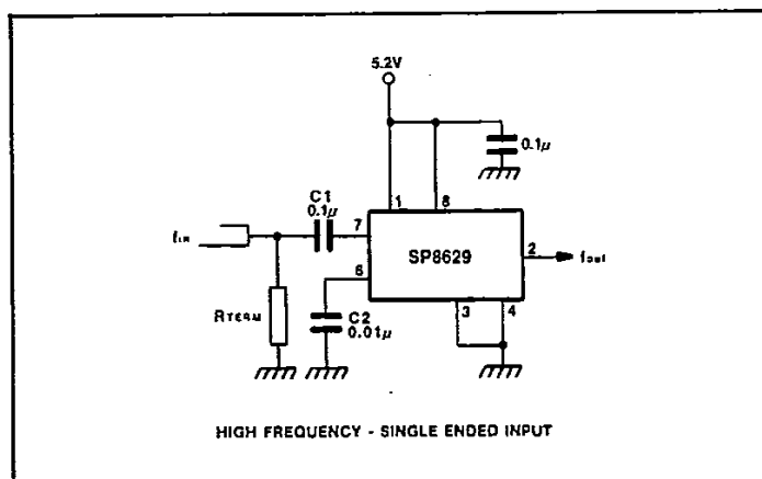
Fig.6 High frequency, single-ended input
