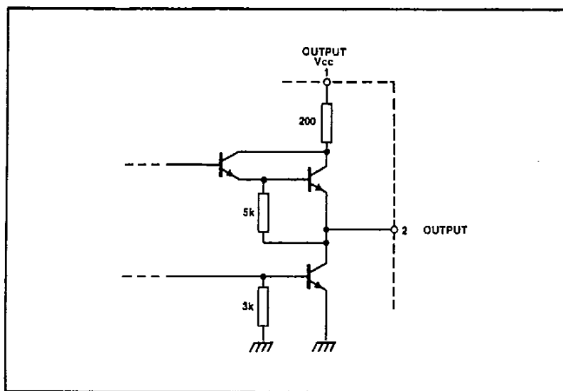
Fig.10 Output circuit diagram
