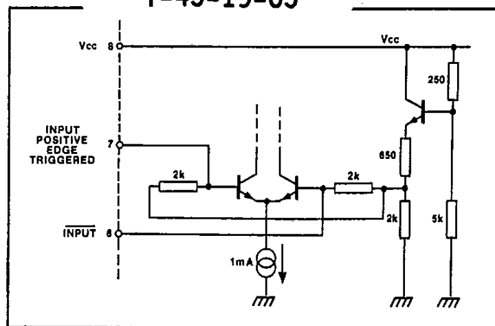
Fig.9 Input circuit diagram
