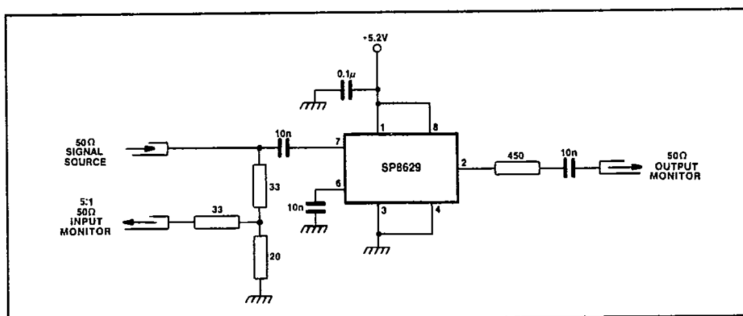
Fig.5 Test circuit
