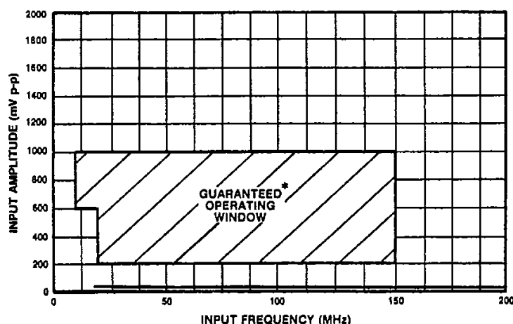
Fig.3 Typical input characteristics SP8629
