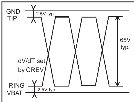
Figure 5. TIP/RING typical ringing waveform
