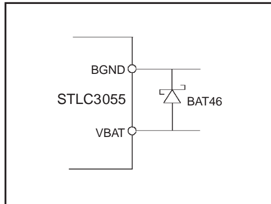
Figure 6. Shottky diode connection
