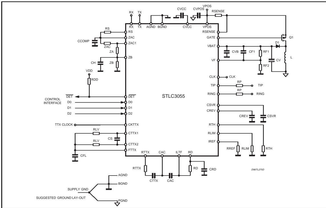
Figure 7. Application Diagram without Metering Pulse Generation.
