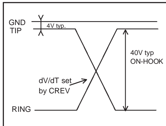
Figure 3. TIP/RING typical transition from Direct to Reverse Polarity
