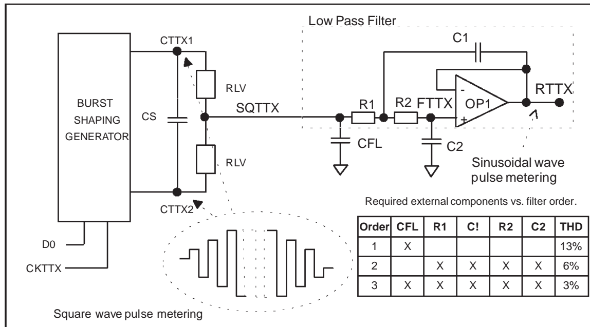
Figure 4. Metering pulse generation circuit.
