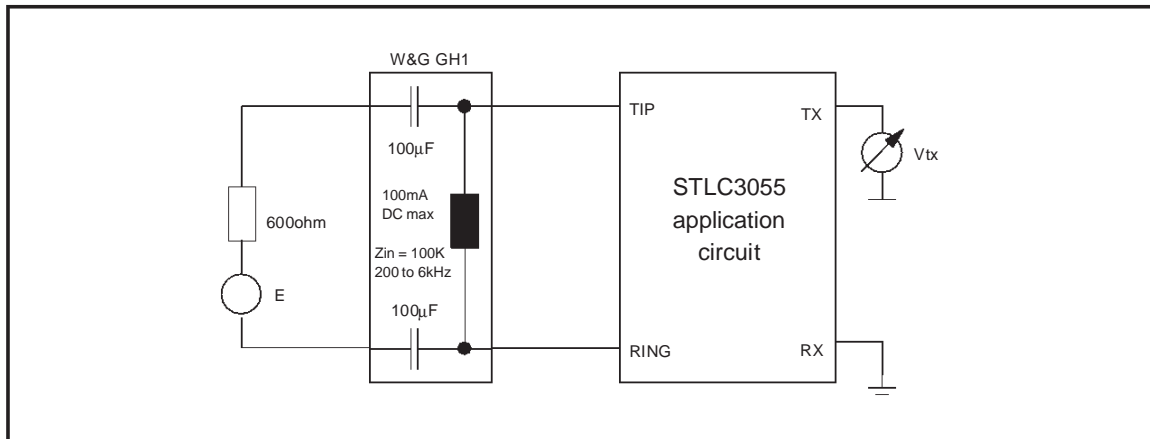
Figure A4. G42 Receive Gain G_{42} = 20\text{Log}|V_I/V_{rx}|
