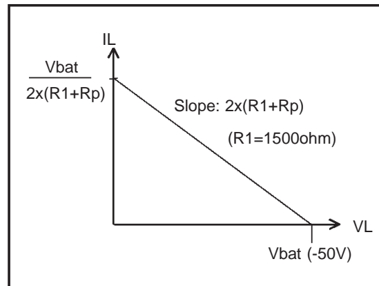
Figure 1. DC Characteristic in HI-Z Mode.
