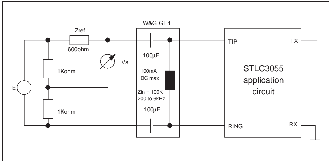
Figure A2. THL Trans Hybrid Loss
