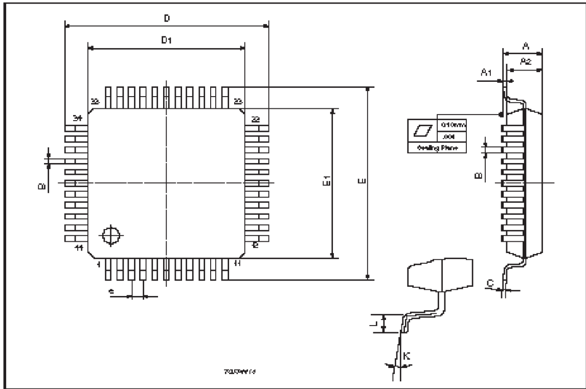
TQFP44 (10 x 10)
