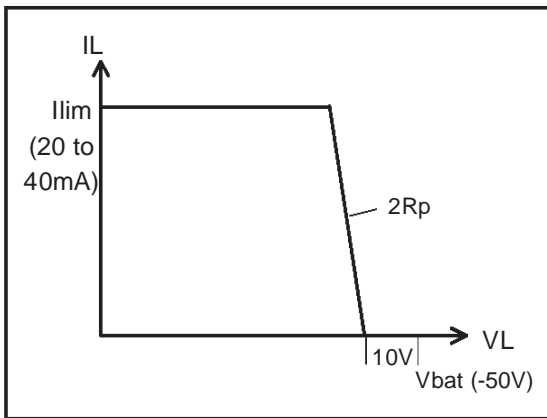
Figure 2. DC characteristic in ACTIVE mode
