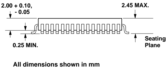
Figure 6. HDMP-0480 Package Drawing.
