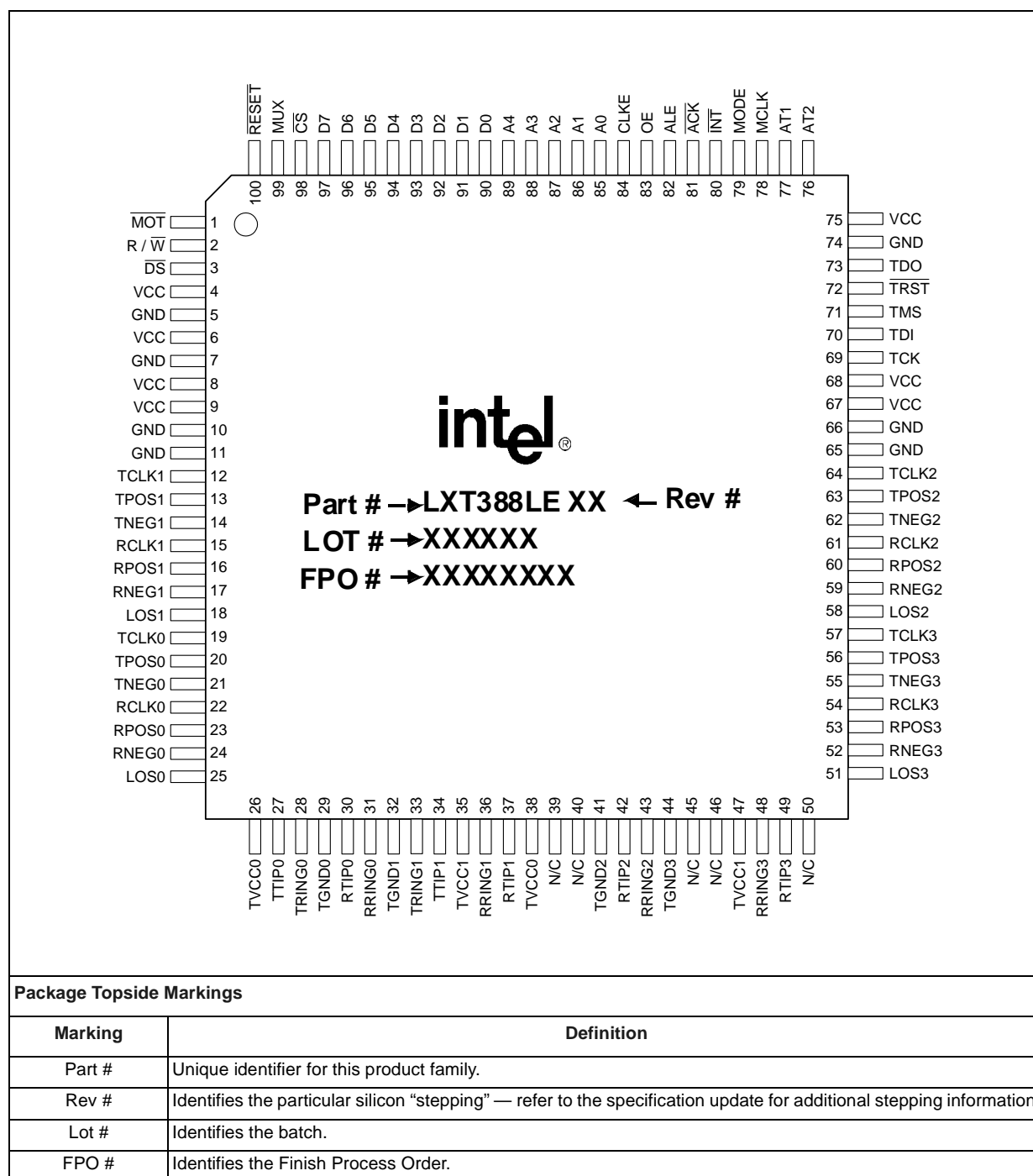
Figure 2. LXT388 Low-Profile Quad Flat Pack Package (LQFP) 100 Pin Assignments and Package Markings
