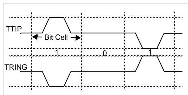
Figure 4. 50% AMI Encoding
