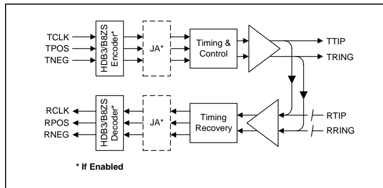
Figure 9. Analog Loopback
