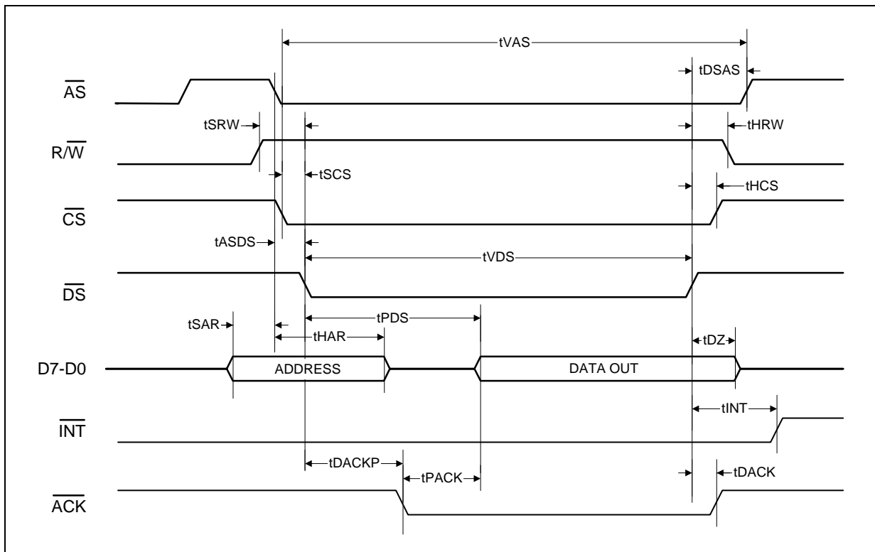
Figure 27. Multiplexed Motorola Mode Read Timing
