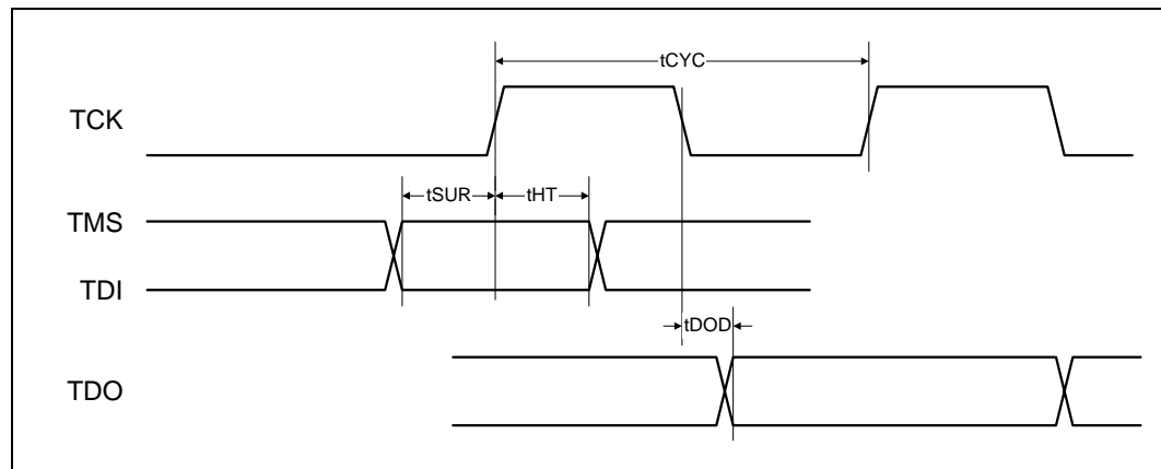
Figure 21. JTAG Timing
