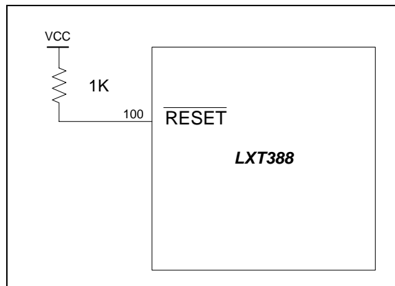
Figure 3. Pullup Resistor to RESET
