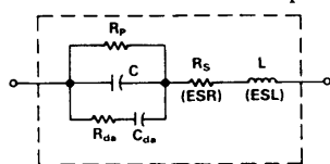
Figure 1. Capacitor equivalent circuit.
