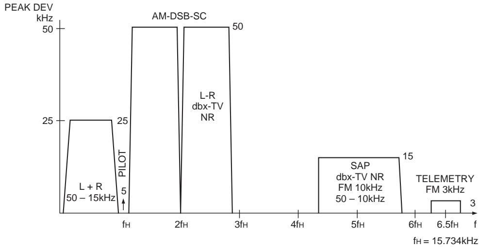
Fig. 1. Base band spectrum
