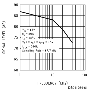
Bipolar Spurious Free Dynamic Range
