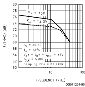
Bipolar Signal-to-Noise + Distortion Ratio vs Input Frequency
