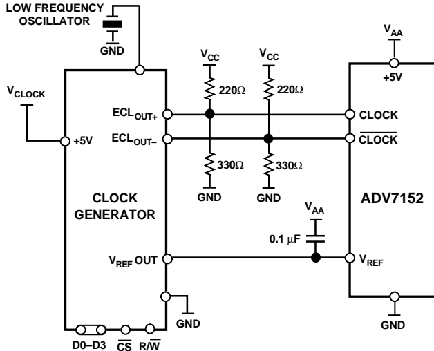
Figure 13. PLL Generator Driving CLOCK, CLOCK of the ADV7152
