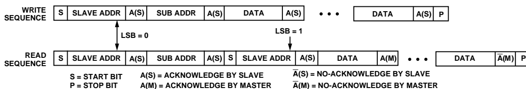
Figure 29. Write and Read Sequences
