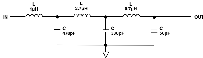
Figure 56. Output Filter
