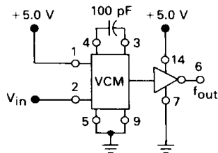
FIGURE 3 — VOLTAGE-CONTROLLED MULTIVIBRATOR
