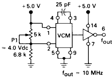
FIGURE 1 — ASTABLE MULTIVIBRATOR
