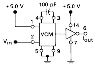
FIGURE 3 — VOLTAGE-CONTROLLED MULTIVIBRATOR
