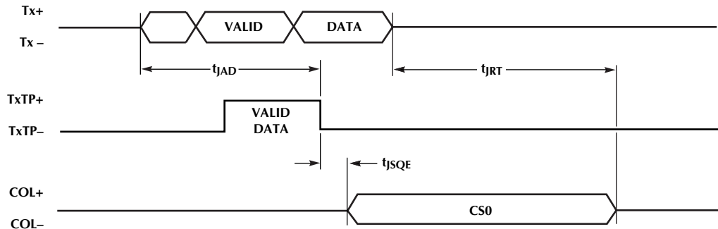
Figure 7. Jabber Timing
