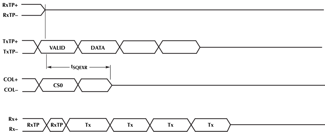
Figure 4. Collision Timing
