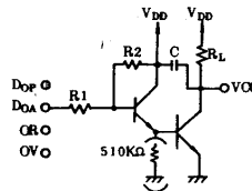
Active filter
