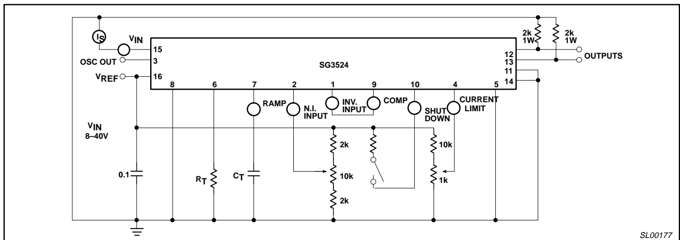
Figure 4. Test Circuit
