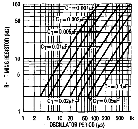
Oscillator Period
