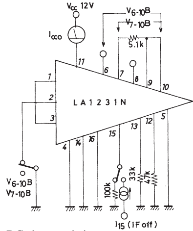
DC characteristics
