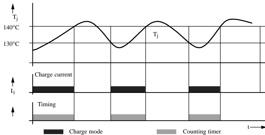
Figure 5. Charge duration – overtemperature
