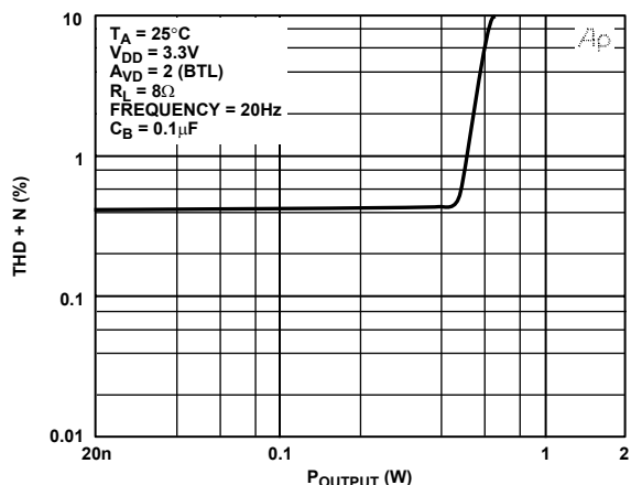
Figure 16. THD + N vs. P_{OUTPUT}
