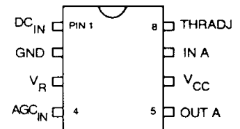
8 PIN PDIP
