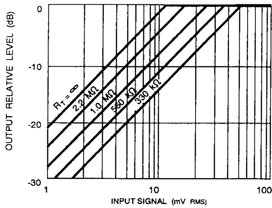
Fig. 2 AGC Characteristics
