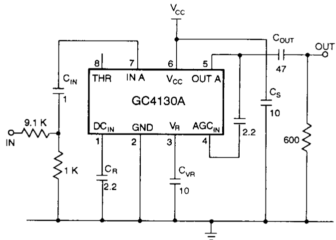
Fig. 6 Test Circuit
