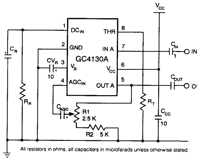
Fig. 8 Maximum Components Circuit
