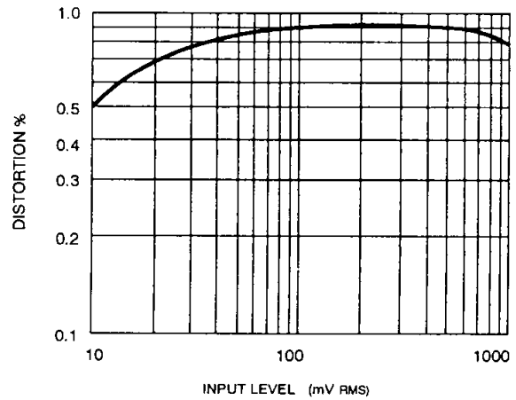
Fig. 5 Distortion Function of Input Level (AGC Mode)
