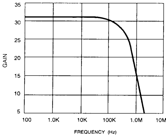
Fig. 4 Amplifier Gain versus Frequency
