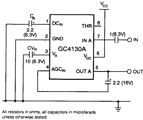
Fig. 7 Minimum Components Circuit
