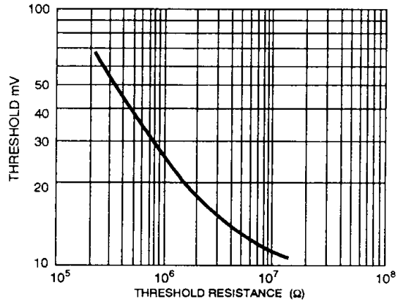
Fig. 3 AGC Threshold versus Resistance ( R_T )
