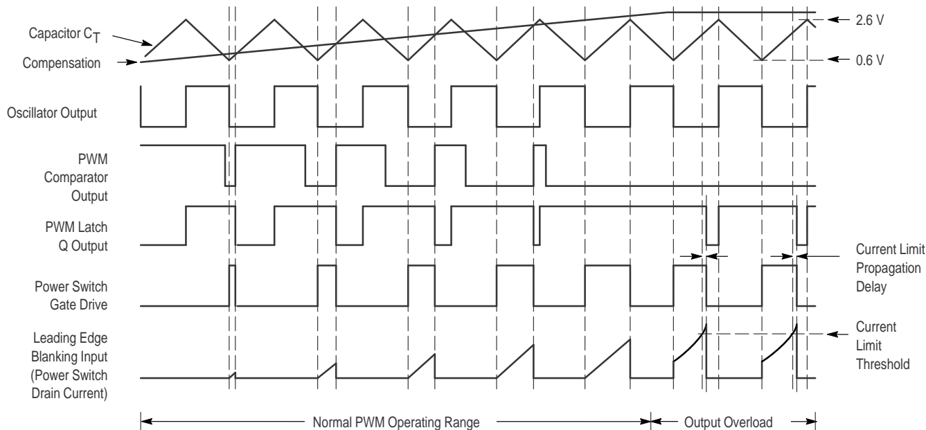
Figure 18. Timing Diagram
