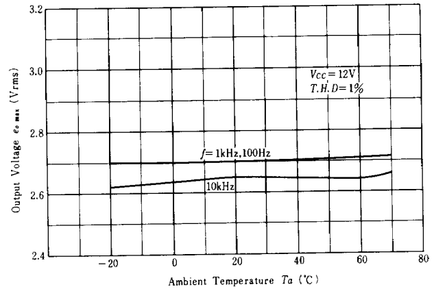
OUTPUT VOLTAGE OF MIC. AMP. VS. AMBIENT TEMPERATURE
