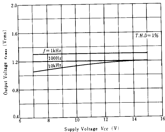
OUTPUT VOLTAGE OF PREAMP. VS. SUPPLY VOLTAGE
