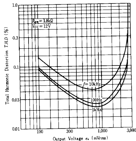
TOTAL HARMONIC DISTORTION OF MIC. AMP. VS. OUTPUT VOLTAGE
