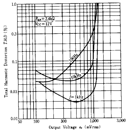
TOTAL HARMONIC DISTORTION OF PREAMP. VS. OUTPUT VOLTAGE
