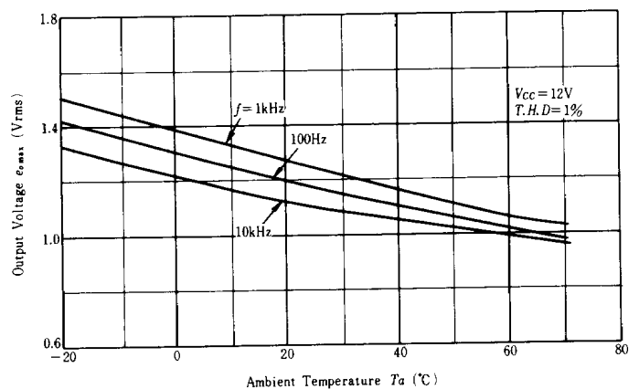
OUTPUT VOLTAGE OF PREAMP. VS. AMBIENT TEMPERATURE
