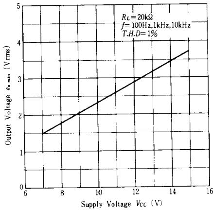
OUTPUT VOLTAGE OF MIC. AMP. VS. SUPPLY VOLTAGE
