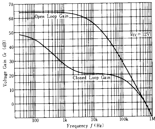
VOLTAGE GAIN OF PREAMP. VS. FREQUENCY
