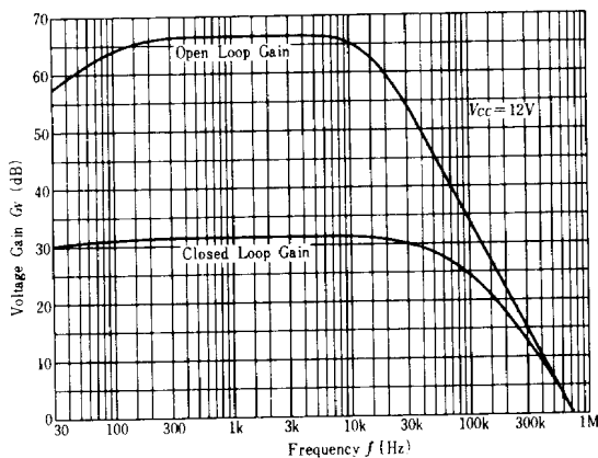
VOLTAGE GAIN OF MIC. AMP. VS. FREQUENCY
