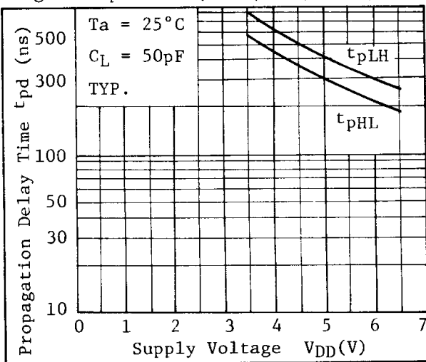
Fig. 9 t_{pd} - V_{DD} (RSEL(H→L)-DATA)
