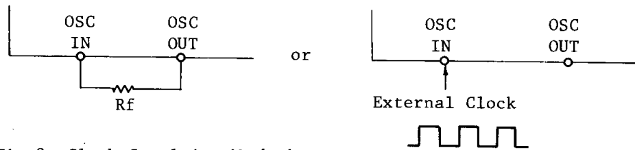
Fig.2 Clock Supplying Methods
