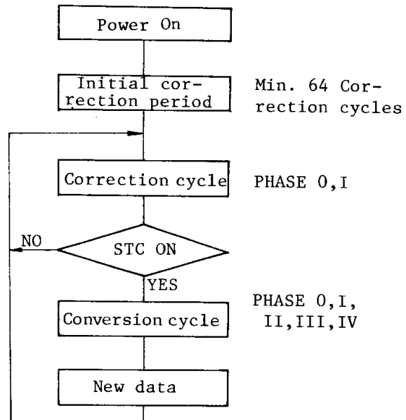
Fig. 1 Operation Flowchart
