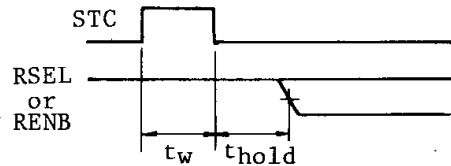
Fig.4 Timing chart of Control Input
