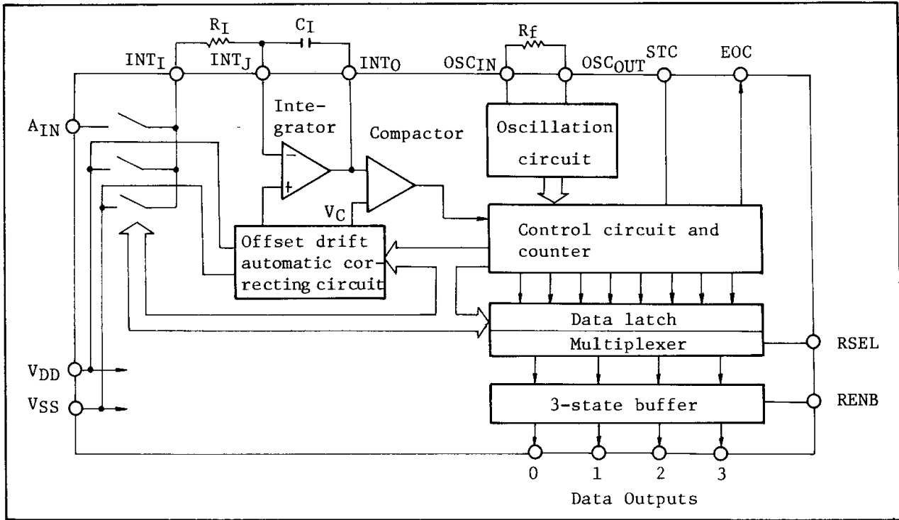
BLOCK DIAGRAM
