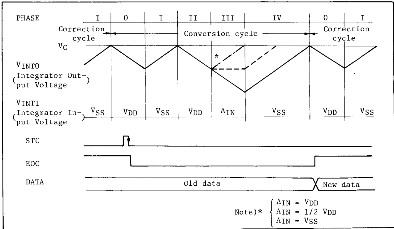
TIMING DIAGRAM
