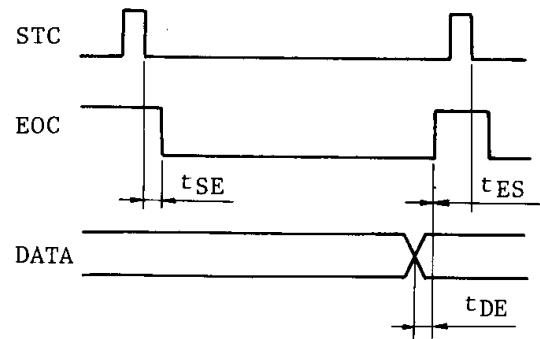
Fig.3 Timing chart of STC/EOC
