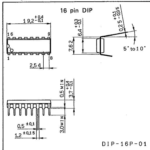
Package Outline
