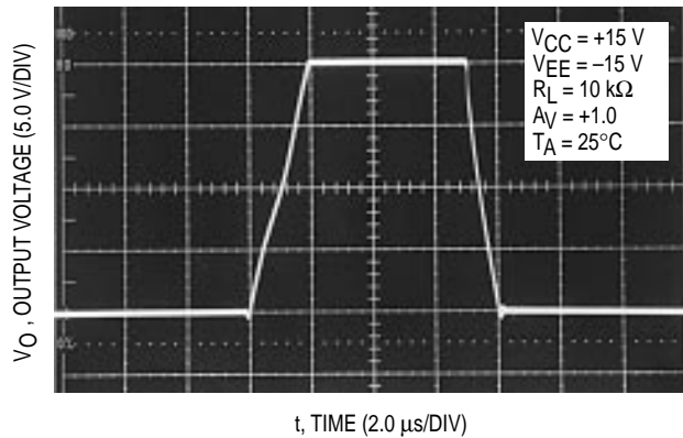
Figure 28. Transient Response
