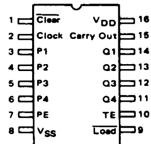
PIN ASSIGNMENT
