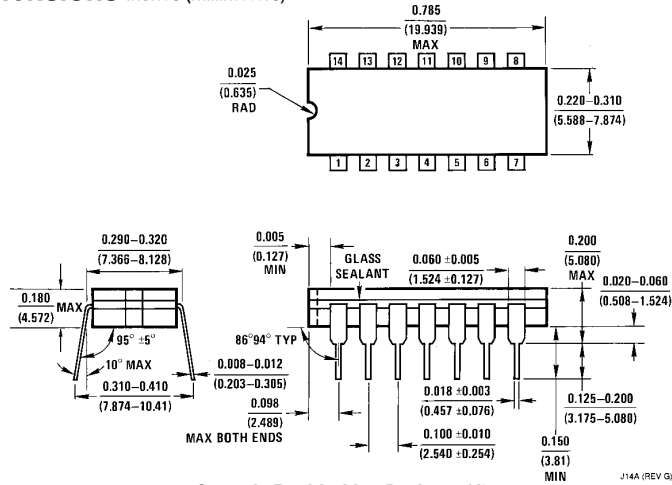
Ceramic Dual-In-Line Package (J) Order Number MM54C85J or MM74C85J NS Package Number J14A
