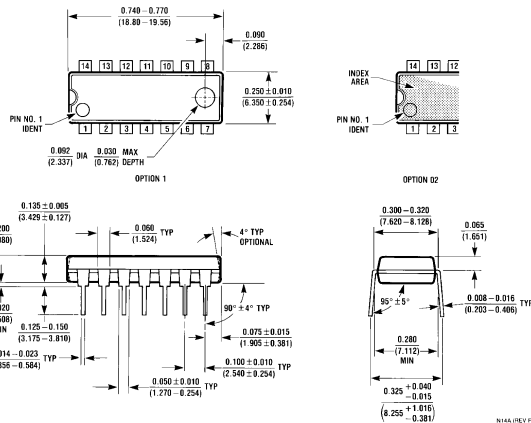
Order Number MM74HC74N NS Package N14A
