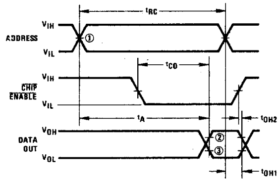
FIGURE 1. Read Cycle
