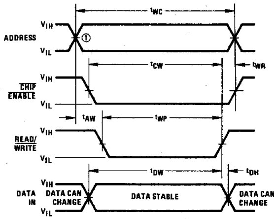
FIGURE 2. Write Cycle
