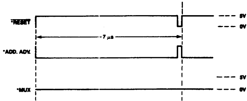
2147H TIMING DIAGRAM 7 μs CYCLE TIME
