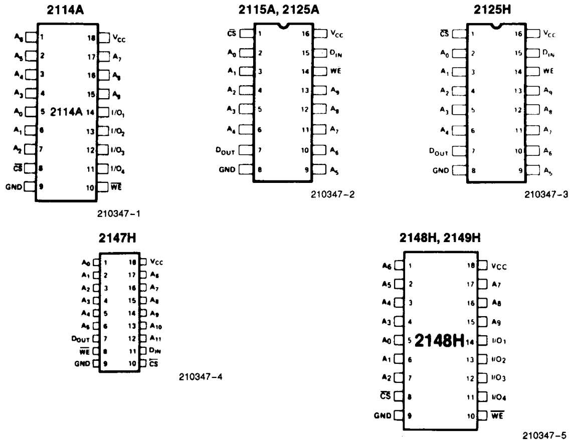
Pin Configuration
