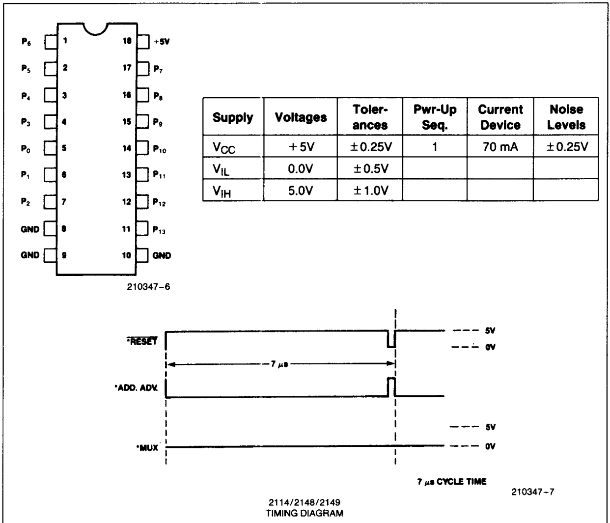
Figure 1. 2114A, 2148H, 2149H Burn-In Configuration
