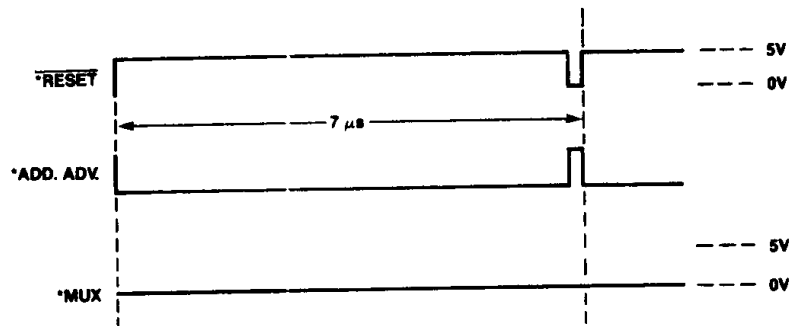
2 | 15/2125 TIMING DIAGRAM 7 μs CYCLE TIME
