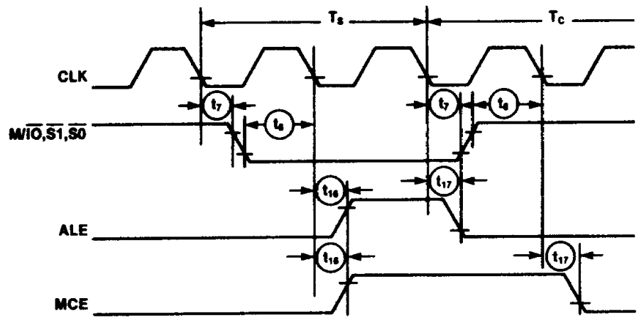
Status, ALE, MCE Characteristics
