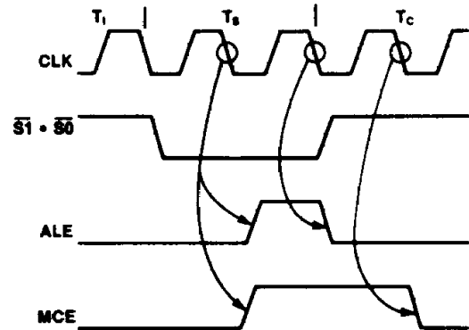
Figure 9. MCE Operation for an \overline{INTA} Bus Cycle
