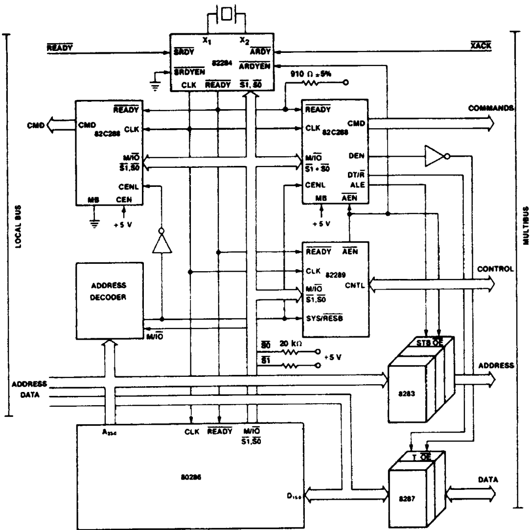
Figure 10. System Use of \overline{\text{AEN}} and CENL
