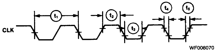
CLK Characteristics
