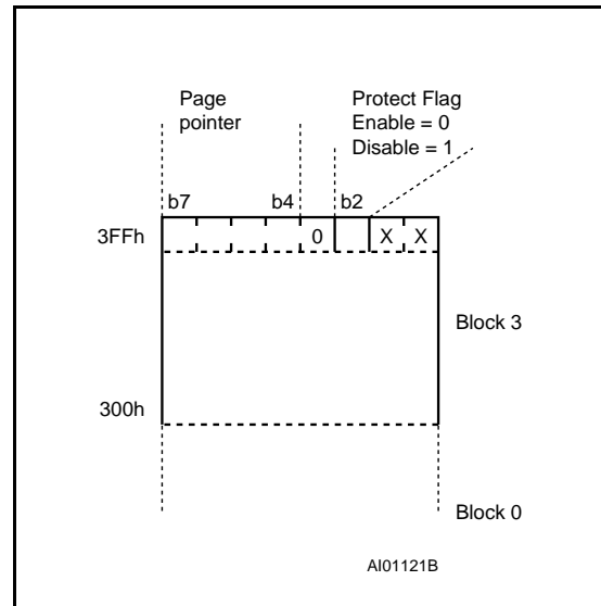
Figure 7. Memory Protection
