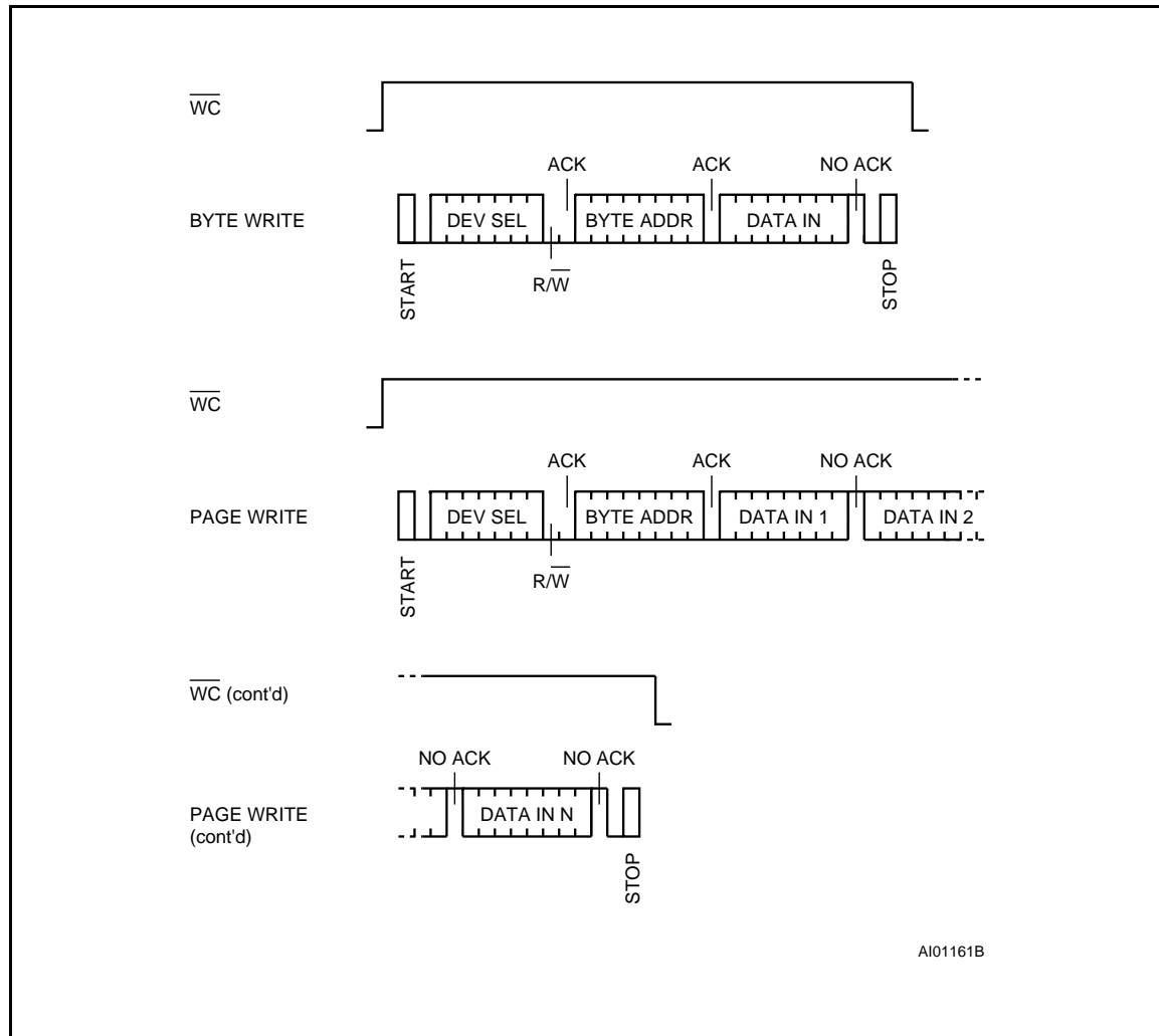
Figure 10. Write Modes Sequence with Write Control = 1 (ST24/25W08)
