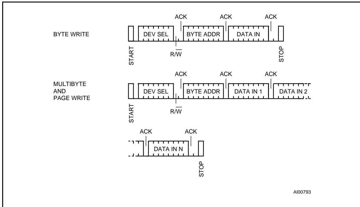
Figure 9. Write Modes Sequence (ST24/25C08)
