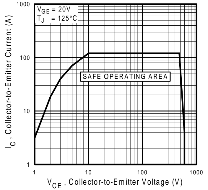
Fig. 12 - Turn-Off SOA
