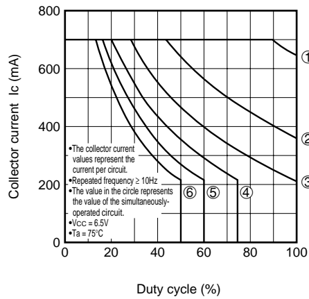
Duty-Cycle-Collector Characteristics
