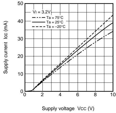
Supply Current Characteristics
