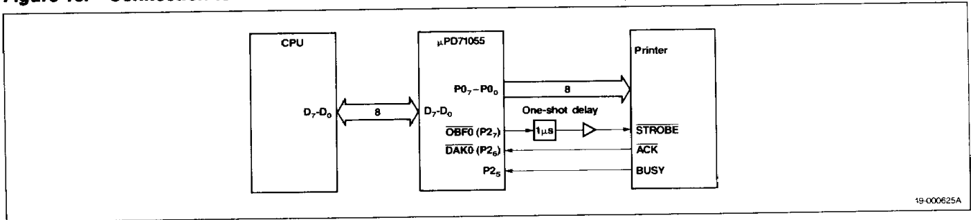
Figure 13. Connection to Printer
