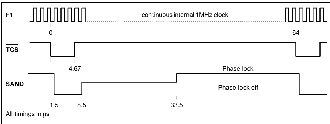
Figure 3 : Synchronization Timing
