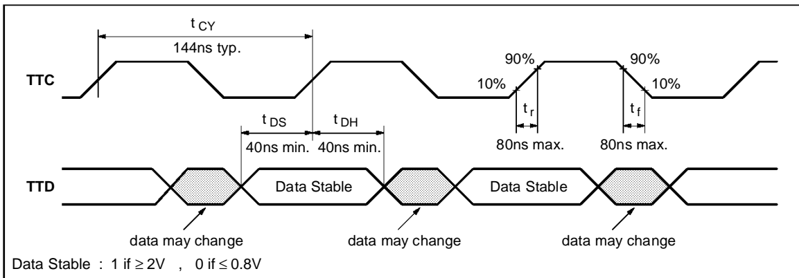
Figure 3 : Synchronization Timing
