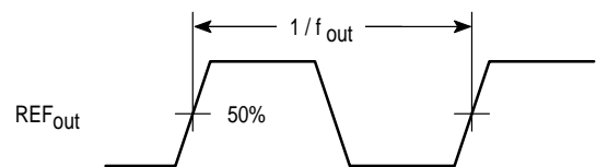
Figure 10. Switching Waveform
