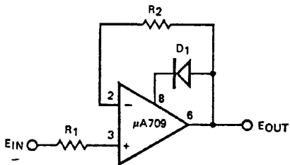
LATCH-UP PROTECTION
