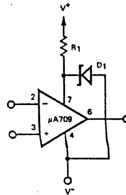
SUPPLY OVERVOLTAGE-PROTECTION
