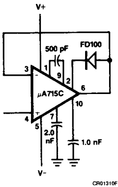
Voltage Follower (Note 1)
