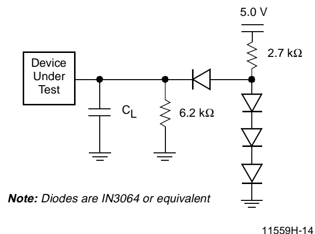
Figure 6. Test Setup
