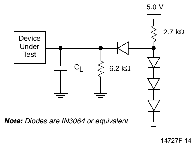
Figure 6. Test Setup
