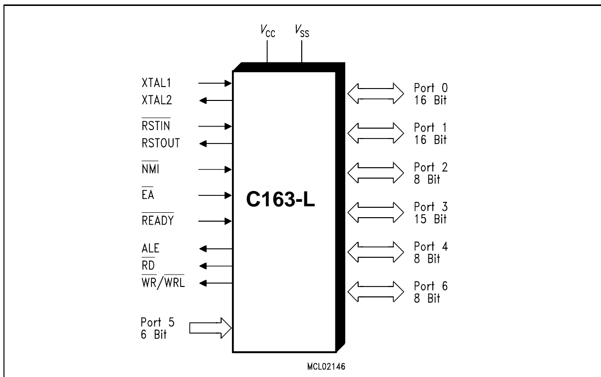
Figure 1 Logic Symbol
