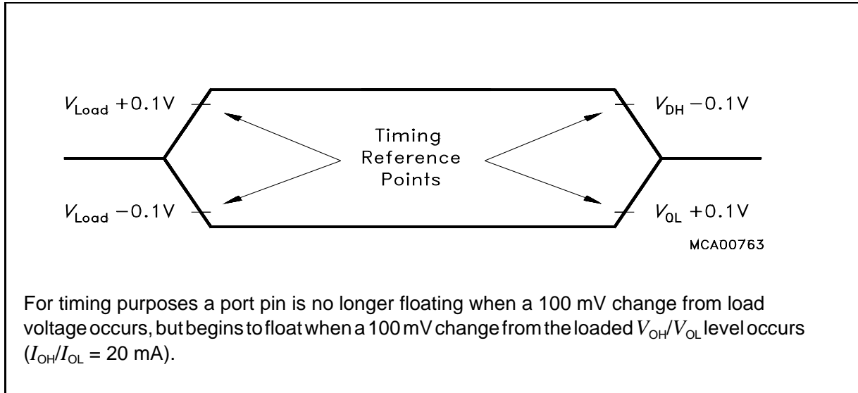
Figure 9 Float Waveforms
