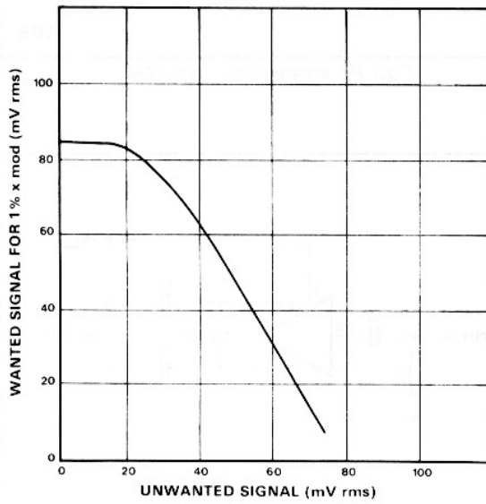
Fig. 4 Cross modulation performance (see note 1)
