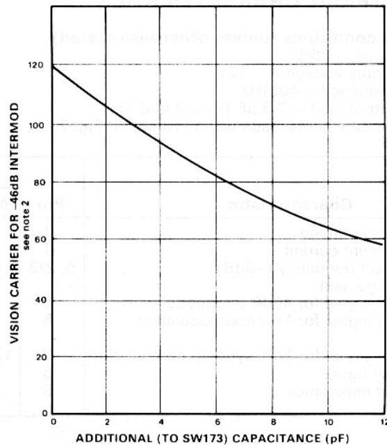
Fig. 7 Intermodulation performance v. load capacitance
