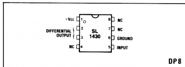
Fig. 1 Pin connections - top view
