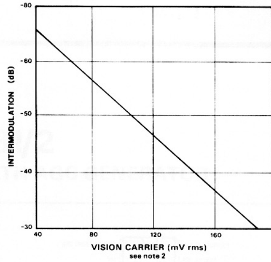
Fig. 9 Intermodulation performance (see note 2)
