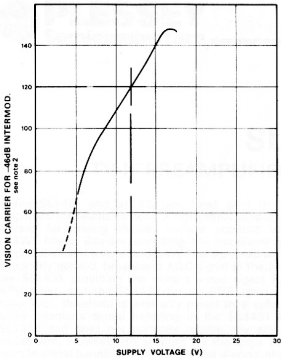
Fig. 8 Intermodulation performance v. supply voltage
