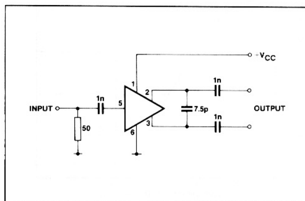
Fig. 2 Test circuit
