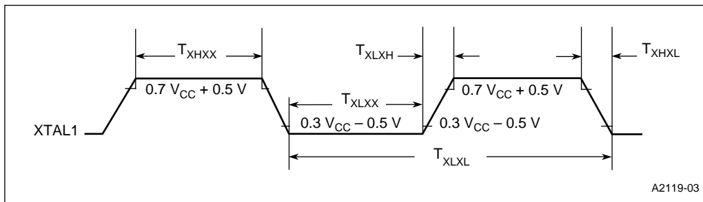
Figure 7. External Clock Drive Waveforms
