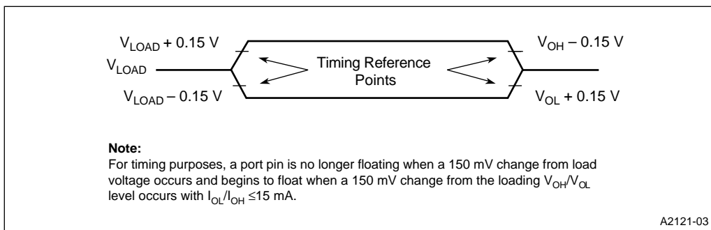
Figure 9. Float Waveforms
