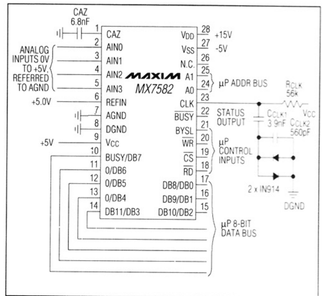
Figure 5. MX7582 Operational Diagram
