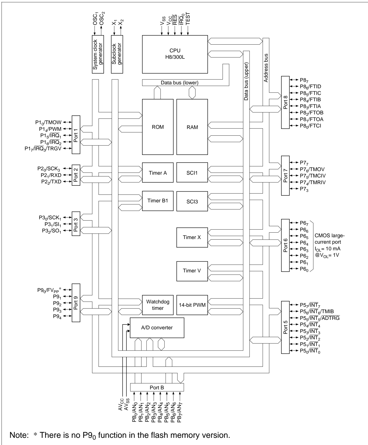
Figure 1.1 Block Diagram
