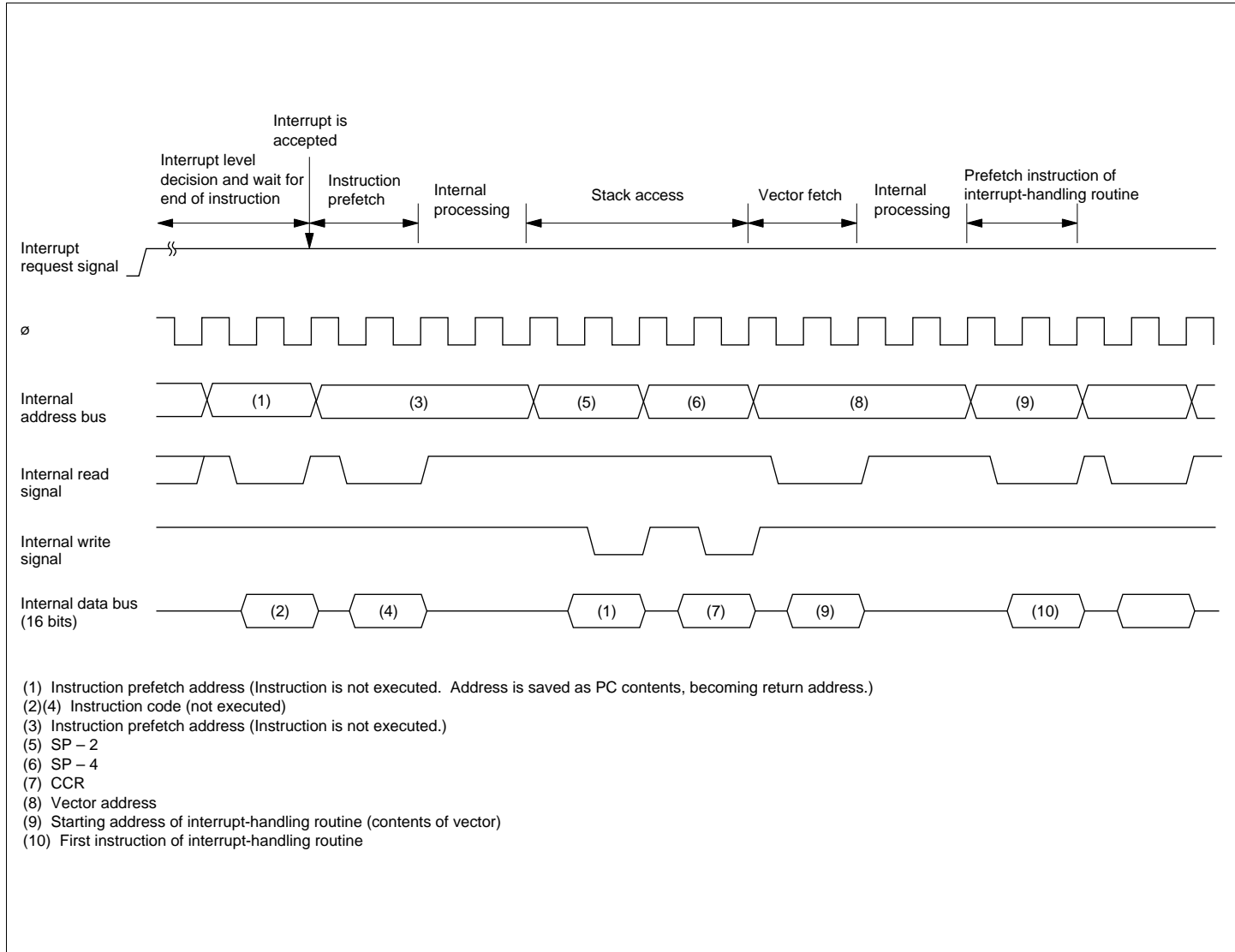
Figure 3.5 Interrupt Sequence
