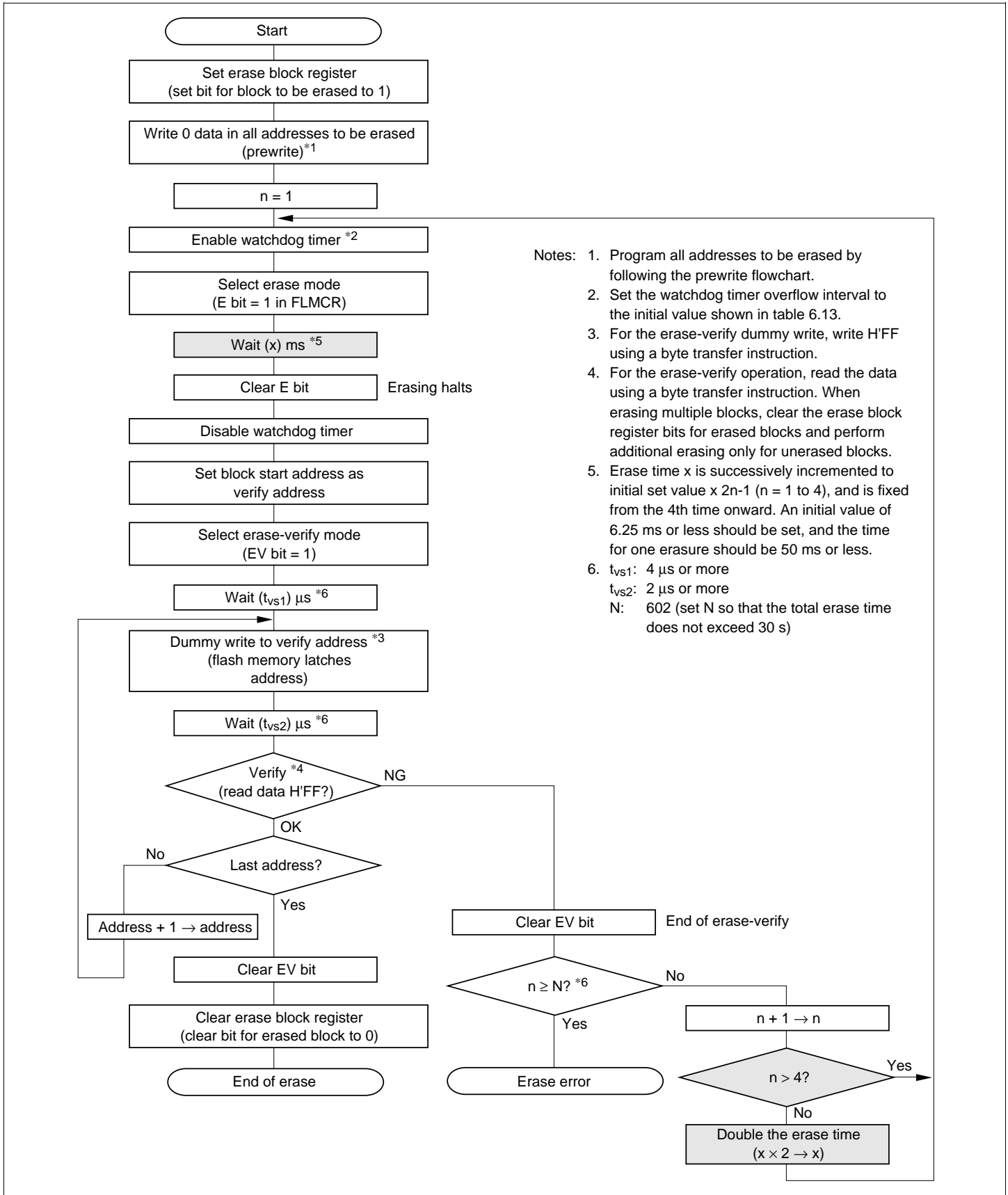
Figure 6.15 Erase Flowchart
